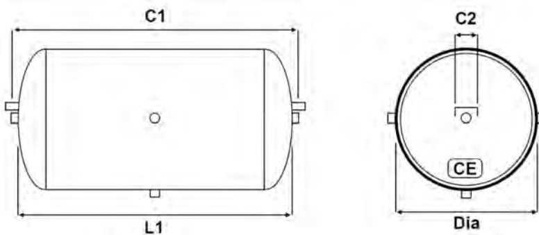
Steel End Mounted 5 Port Reservoirs
